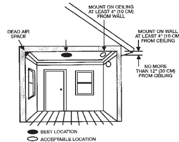
Figure 5: RECOMMENDED SMOKE ALARM MOUNTING LOCATIONS
